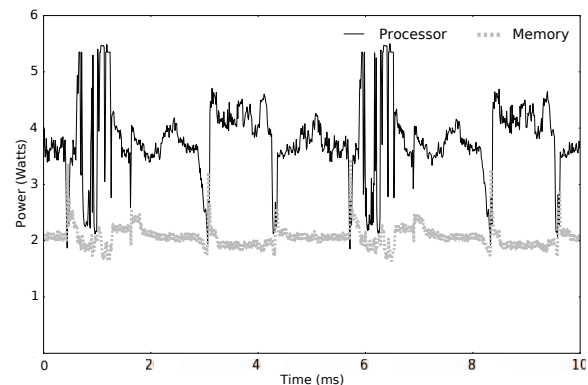
Fig. 1: Time variation of the power consumed by the processor and memory dies of a 3D stack for the MG benchmark of NAS with 8 cores.
